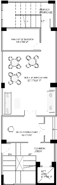
GROUND FLOOR
