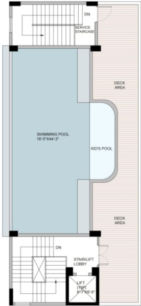
ROOF TOP PLAN
