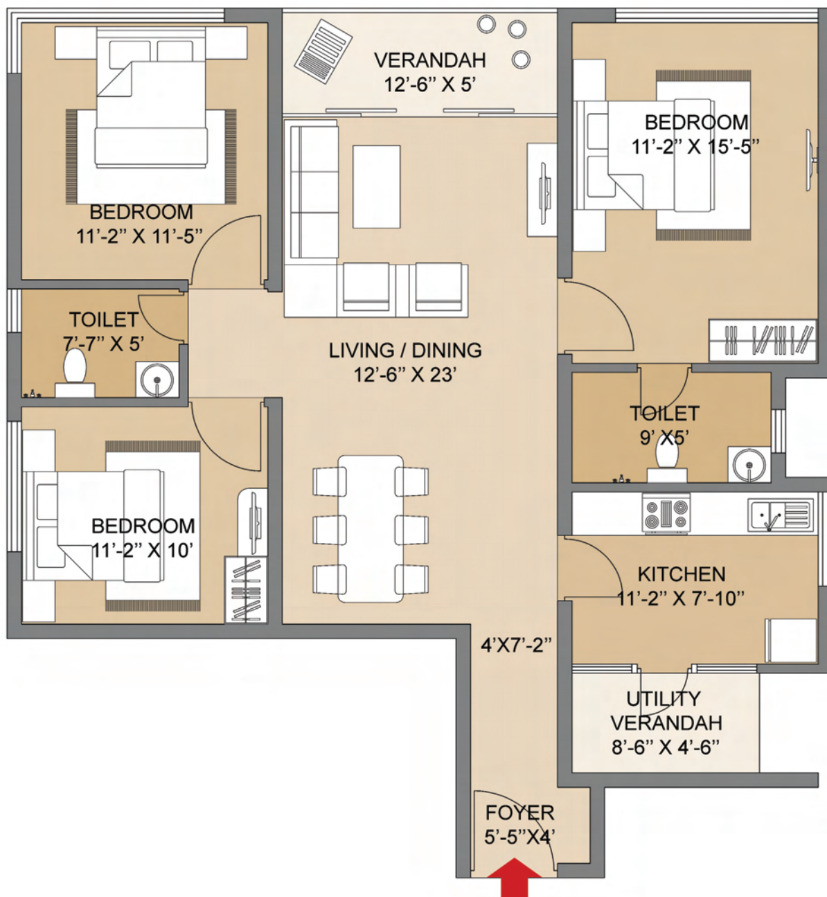
Type 3S - 1512 sq ft
